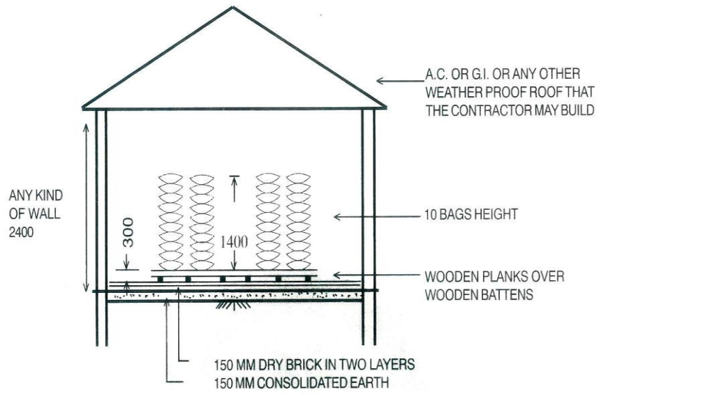
SECTION AB
